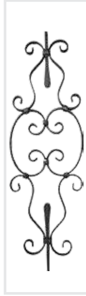
▶M-68 H.800xL.250mm ∅12
